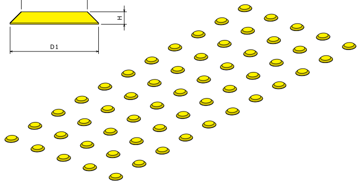
WARNING STUDS IN DIAGONAL ARRANGEMENT, VERTICAL AND ISOMETRIC VIEW
